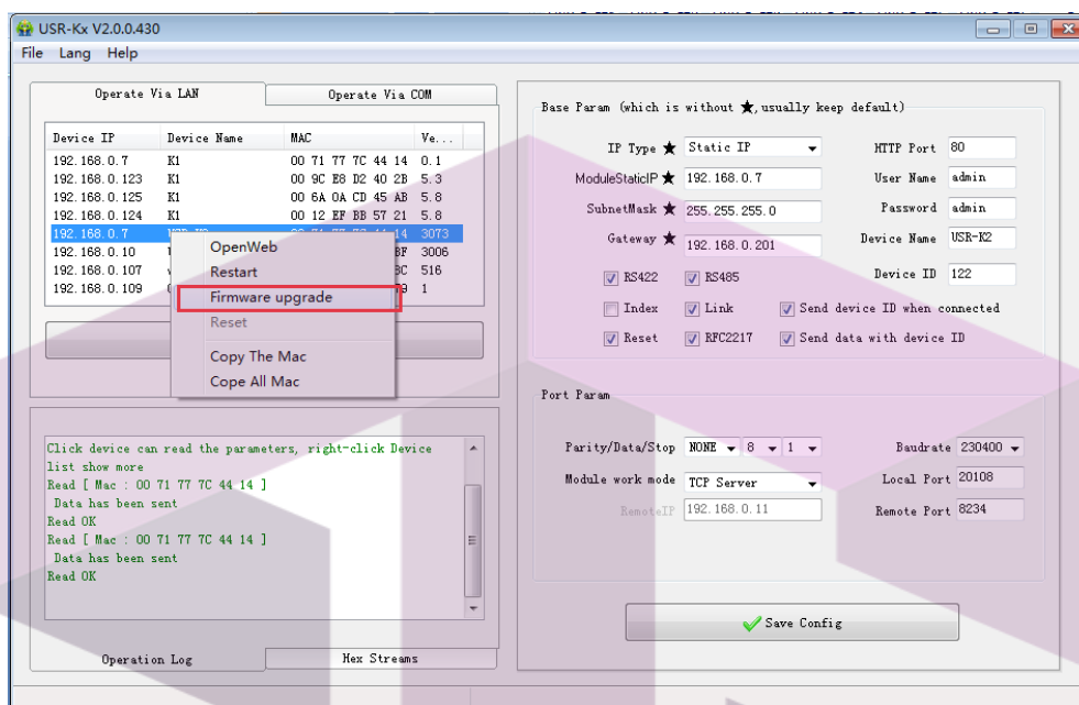
Diagram4-9 Setting Software
