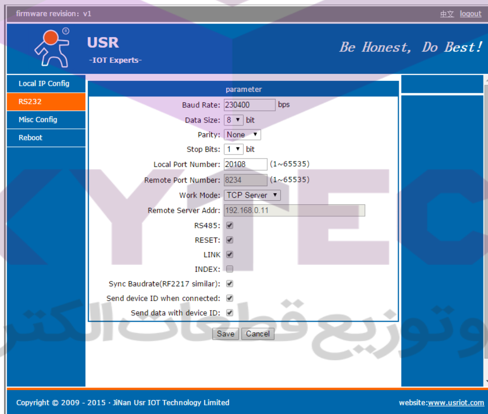
Diagram 4-3 Web—RS232
